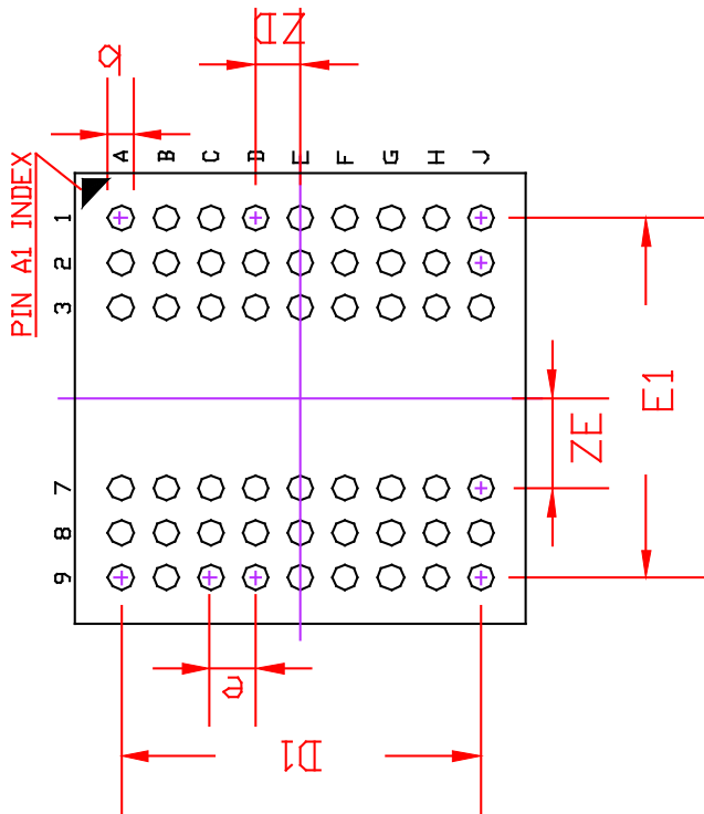
BOTTOM VIEW
